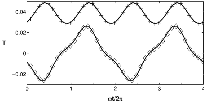
FIG. 16. The temporal variation ( simulation ) of linear eigenvectors multiplied with adjusted amplitude factors A=0.0382 , B=0.0108 (see text) at \delta Fr=3.732 \times 10^{-4} , R=4790 for the harmonic (upper curve) and subharmonic (lower curve) modes, respectively. Comparison is made with the numerical amplitudes of the Fourier modes at \mathbf{q}_1^H (+) and \mathbf{q}_1^S ( \diamond ), respectively, for the SQC midplane temperature field T(\mathbf{x}, t) \equiv \Theta(\mathbf{x}, z=1/2, t) in units of \Delta T .
